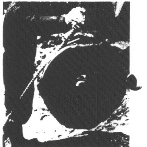
Fig. 2. A massive, 18 \frac{3}{4} -in., 10,000-psi by 26 \frac{3}{4} -in., 5,000-psi casing spool (and enclosed 13 \frac{3}{8} -, 10 \frac{3}{8} -, 7 \frac{3}{8} - and 3 \frac{1}{2} -in. tubulars) was cut in 4 hours using the Hytorc cutter.
