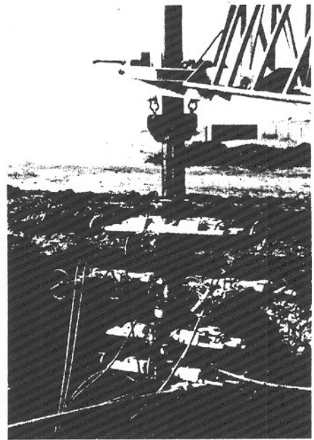
The capping assembly is lowered to the top of 9-in., swallowing 48 in. of 7-in. casing. Top of 7-in. will be located just below valving area of the kill spool. Inverted pipe rams and the 7-in. slip rams are closed and locked, connecting the capping assembly to the 7-in. casing. Pump lines are connected and tested before closing well in. The well can now be killed. Due to the nature of the annular dual completions in these wells, the stack will be left in place for a few days of lubricating (bleed off pressure that may have built up and circulate more kill fluid as needed) while another well is being prepared. After removing BOP stack, a 7-in. socket-weld flange and 3,000-psi ball valve are installed. The well is temporarily secure and can be put back on production as equipment becomes available.
