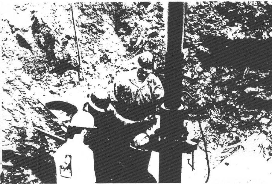
Once 9-in. is exposed, three cuts of approximately 16 in. each are made using pneumatic air cutter to expose 48 in. of 7-in. casing. A brass hammer was used to jar the 9-in. casing and fracture cement between it and the 7-in. casing to facilitate removal of the 9-in. With 48 in. of 7-in. casing exposed, the well is ready for capping.
