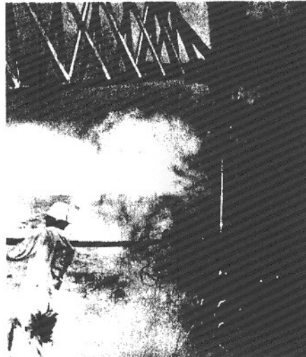
Once 9-in. is exposed, three cuts of approximately 16 in. each are made using pneumatic air cutter to expose 48 in. of 7-in. casing. A brass hammer was used to jar the 9-in. casing and fracture cement between it and the 7-in. casing to facilitate removal of the 9-in. With 48 in. of 7-in. casing exposed, the well is ready for capping.
